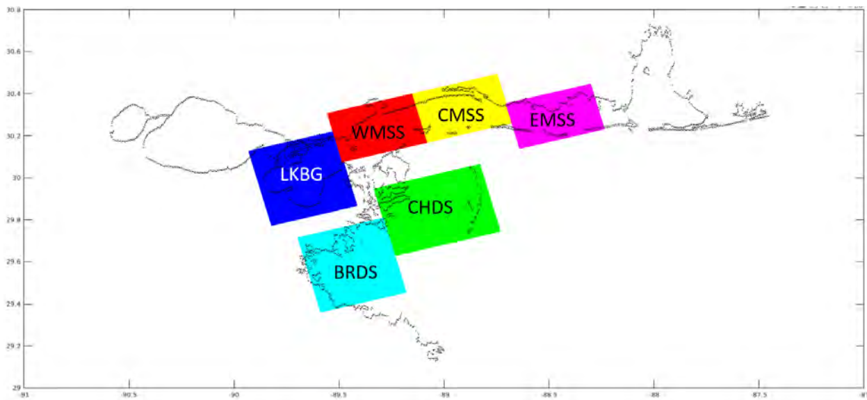
Figure 14-2. Bounding boxes used to calculate area statistics for salinity. Abbreviations are as follows for the six ROIs: LKBG=Lake Borgne, WMSS=Western Mississippi Sound, CMSS=Central Mississippi Sound, EMSS=Eastern Mississippi Sound, CHDS=Chandeleur Sound, and BRDS =Breton Diversion/Sound.
