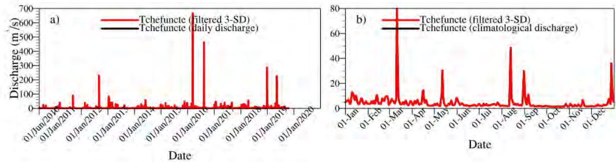
Figure A23: Interannual daily river discharge data for the Tchefuncte River (Station 07375000) (a) and the corresponding daily climatological discharge (b).
