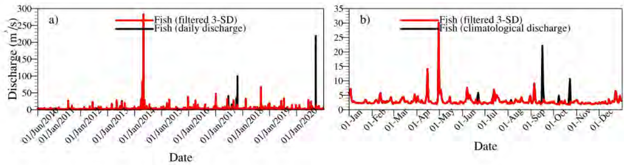
Figure A7: Interannual daily river discharge data for the Fish River (Station 02378500) (a) and the corresponding daily climatological discharge (b).
