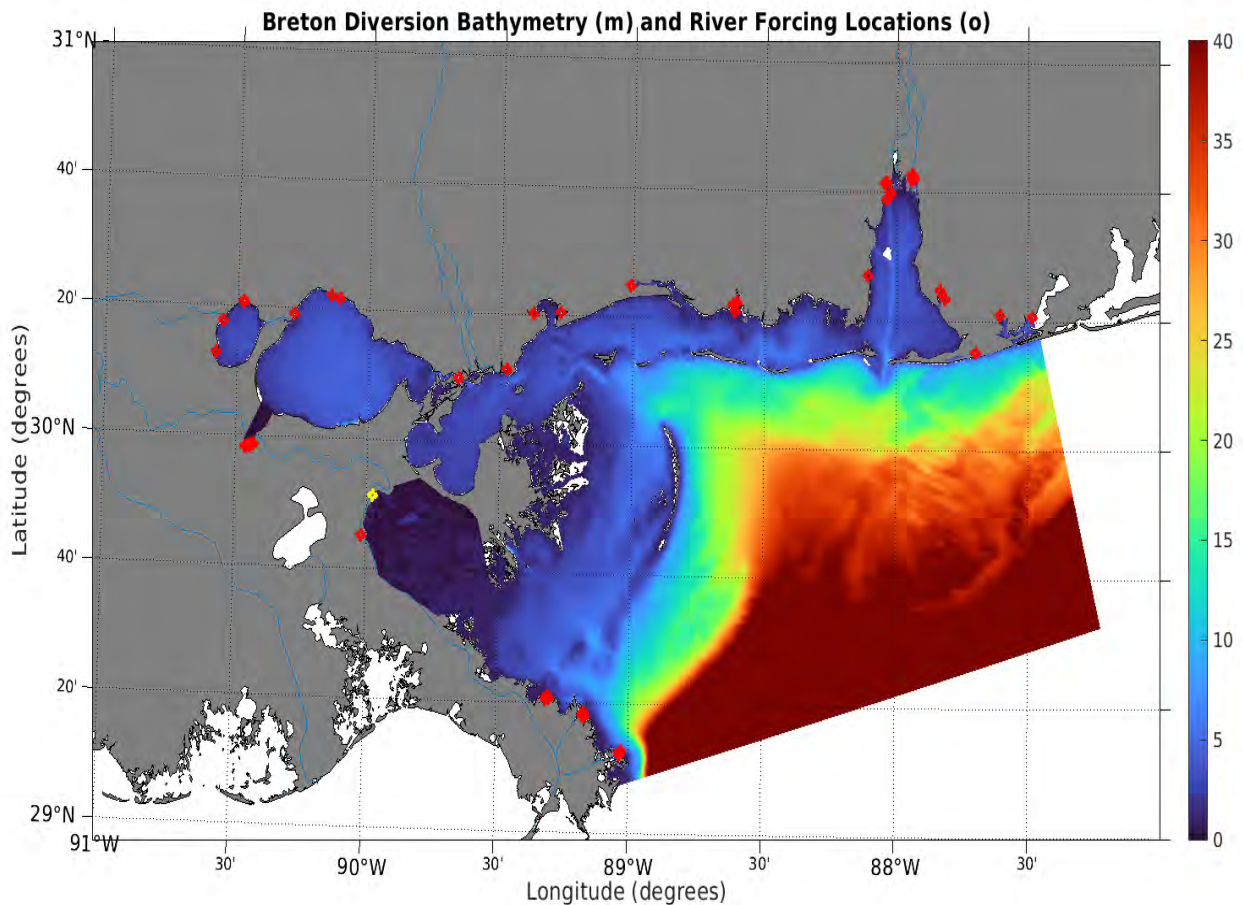
Figure 5. The msbCOAWST grid bathymetry in meters for the model domain. River inflow locations into the msbCOAWST domain are marked as red circles. River names and their USGS gauge station IDs are noted in Figure A1 and Table A1, respectively. Further details of these river discharge locations and applied processing methods are provided in the Appendix. The location of the USGS gauge station at Belle Chasse is marked as a yellow circle. The three discharge locations along the Birdfoot Delta that flow directly into the WMSS are set to discharge 10%, 12.5% and 10% of the total MS River discharge at Belle Chasse. The bathymetry applied for this modeling application is drawn from the NGCHC 3 arc second DEM (Wiggert et al., 2018). The applied datum for this DEM is NAVD88.
