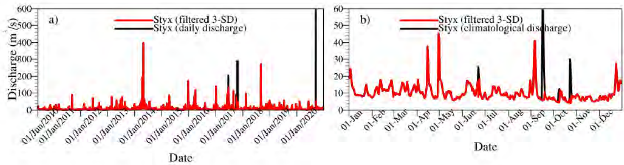
Figure A4: Interannual daily river discharge data for the Styx River (Station 02377570) (a) and the corresponding daily climatological discharge (b).
