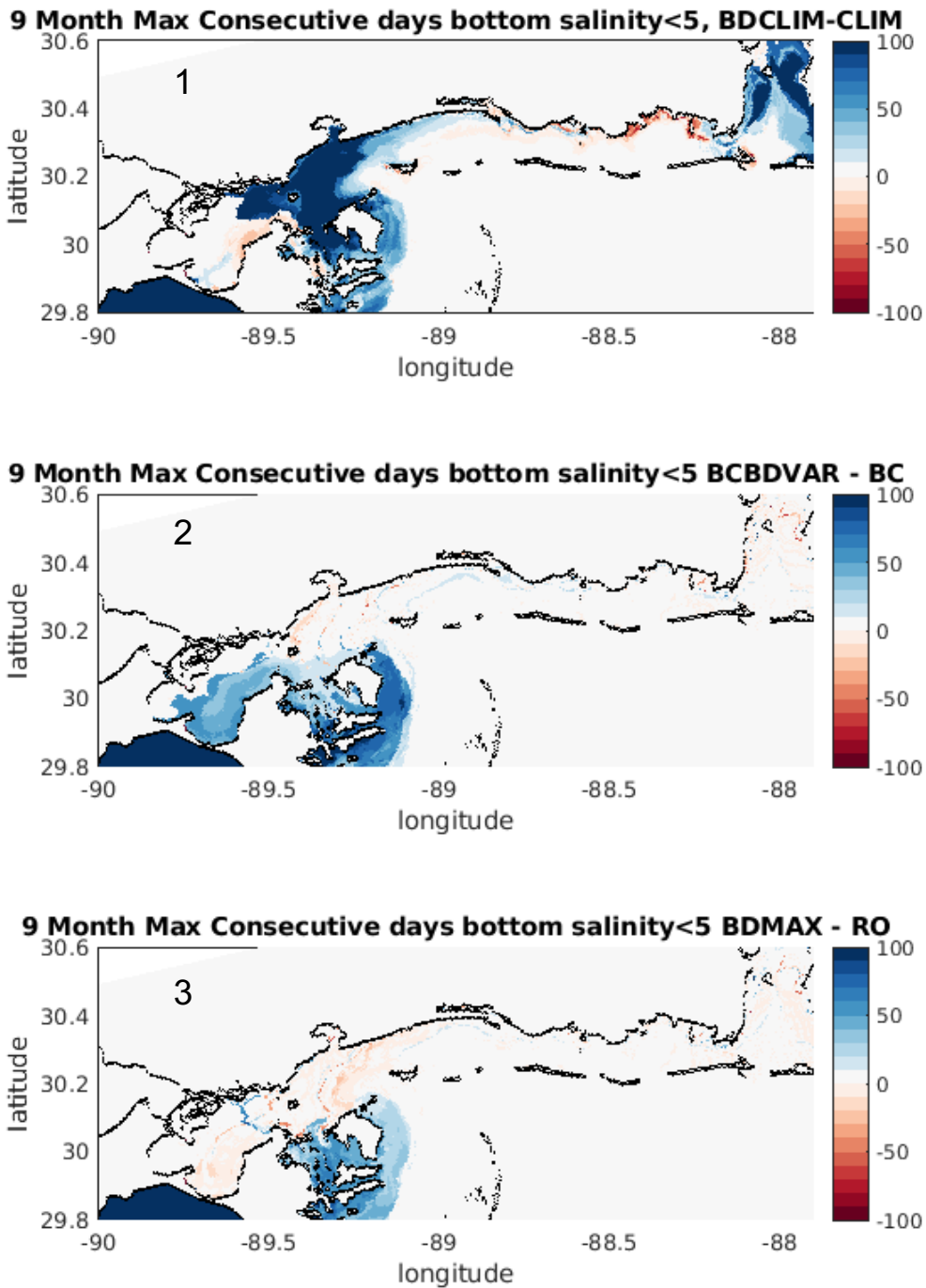
Figure 19. Difference in the maximum consecutive days where average bottom salinity is below 5 ppt (across twin experiments, Table 4) between scenarios with and without active Breton Diversion. Positive values (blue, fresher) indicate there are more consecutive days below 5 ppt when the Breton Diversion is active, while negative values (red, saltier) indicate there are less consecutive days below 5 ppt.
