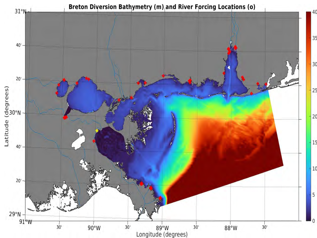
Figure E1. The USM ocean modeling system applied to assess potential impacts from the Mid-Breton Sound Diversion accounts for coastal water depth levels (bathymetry) in meters (see color legend) and for freshwater inflows from surrounding rivers (red diamonds) and the Bonnet Carré Spillway using data from the USGS gauge station at Belle Chasse (yellow diamond).
