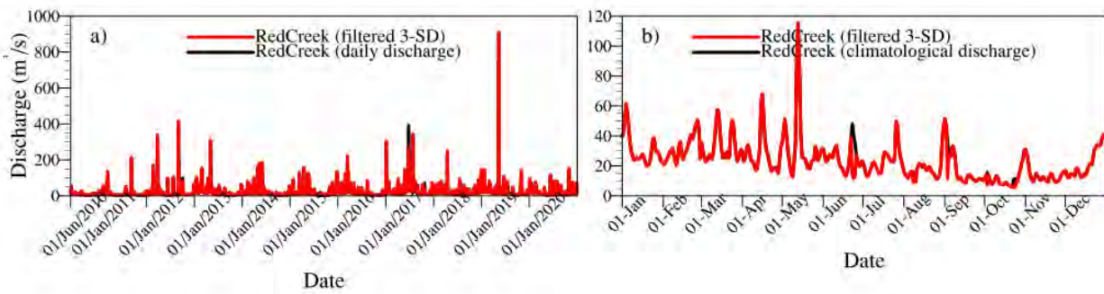
Figure A12: Interannual daily river discharge data for the Red Creek (station 02479300) (a) and the corresponding daily climatological discharge (b).
