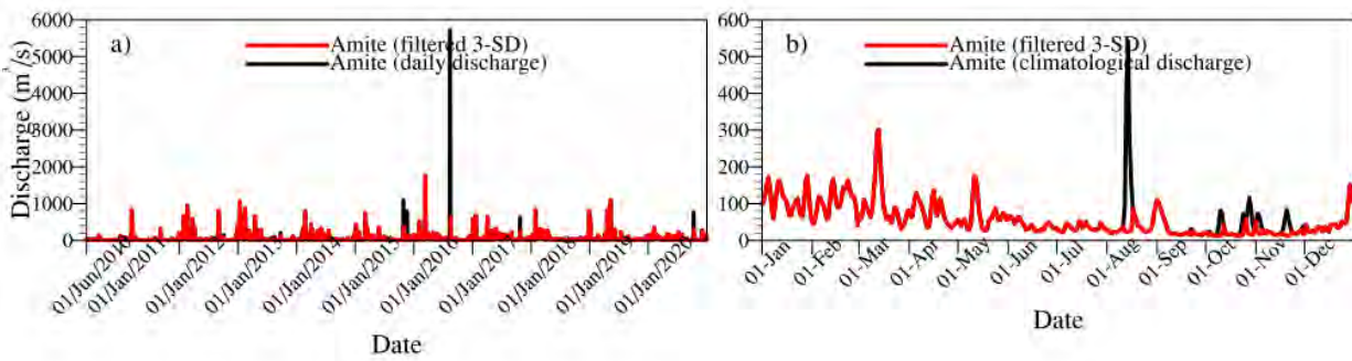
Figure A18: Interannual daily river discharge data for the Amite River (Station 07378500) (a) and the corresponding daily climatological discharge (b).
